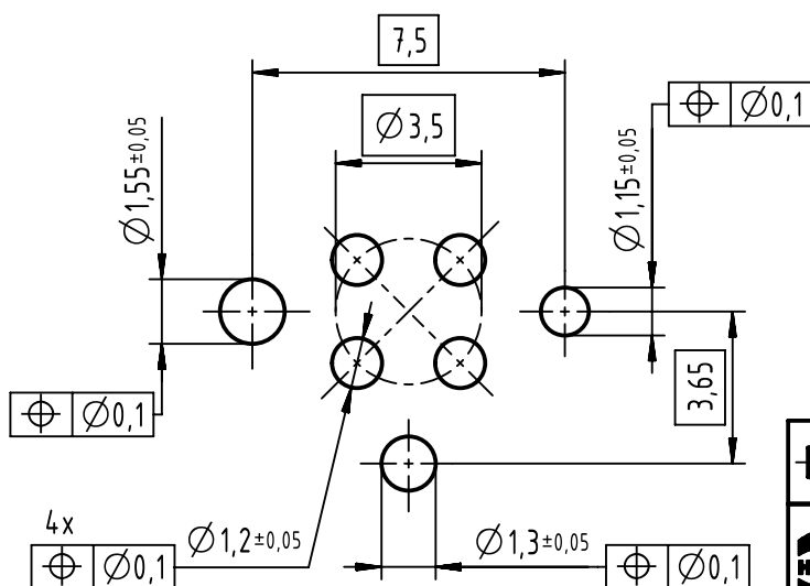
recommended PCB layout A (5:1)
